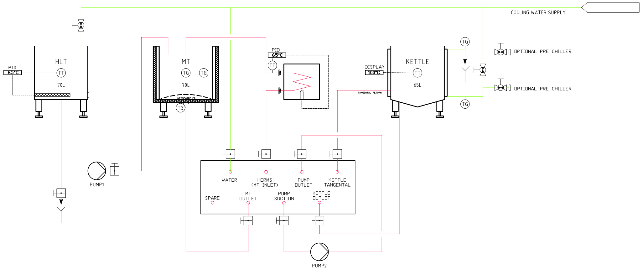
MASH RECIRCULATION
