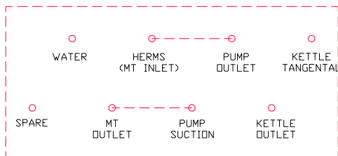
MASH RECIRCULATION
