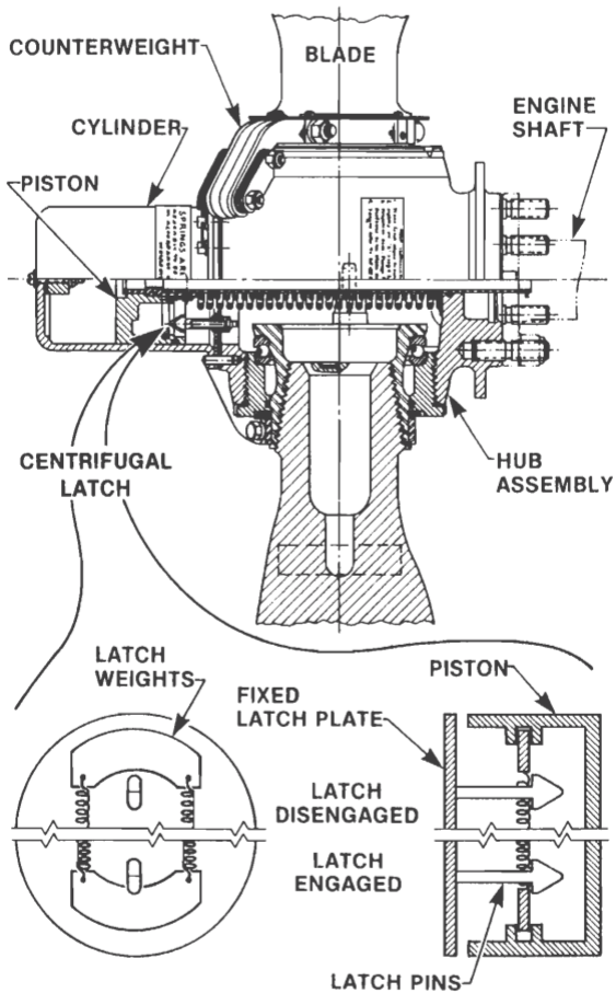
Figure 4-5. A version of the centrifugal latch mechanism used to prevent a feathering propeller from feathering when the engine is shut down on the ground.
