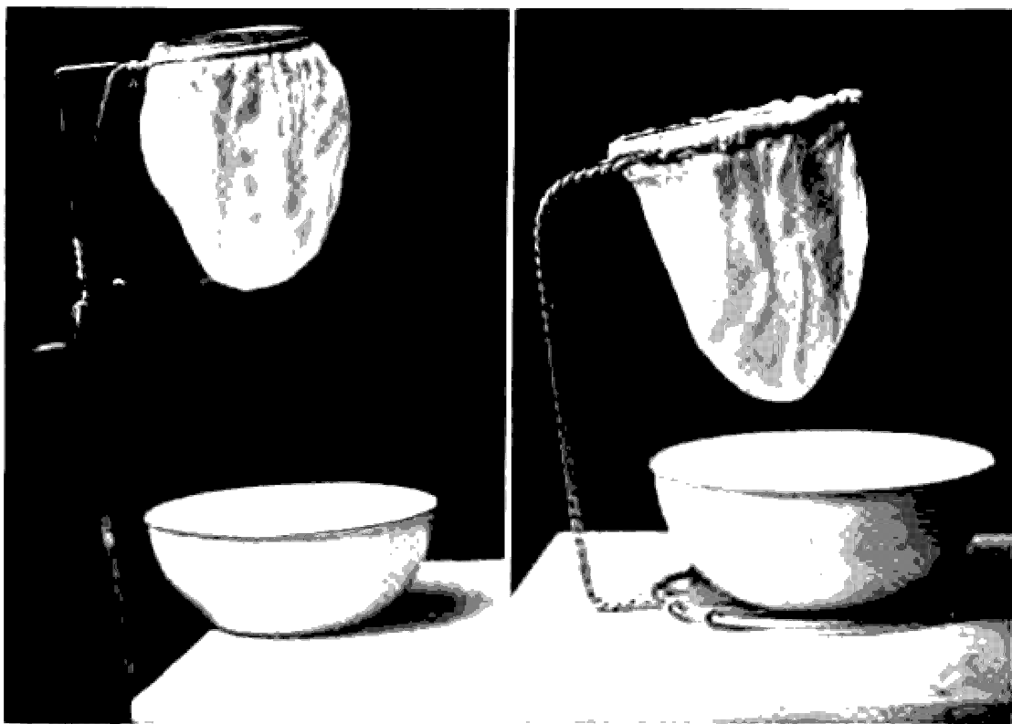
FIG. 97.—A commercial jelly strainer placed on a chair back.
