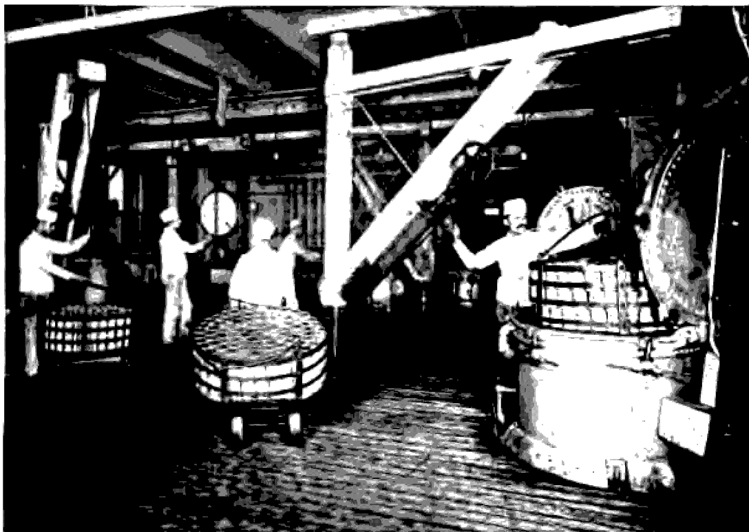
FIG. 66.—Commercial retorts where steam is piped in from the boiler. (Heins Company)
