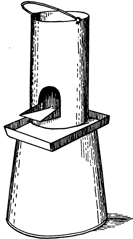
10. 29 - fire-pot for roasting corn-cobs for heating tools. A gasoline fire-pot or charcoal bucket may also be used.
