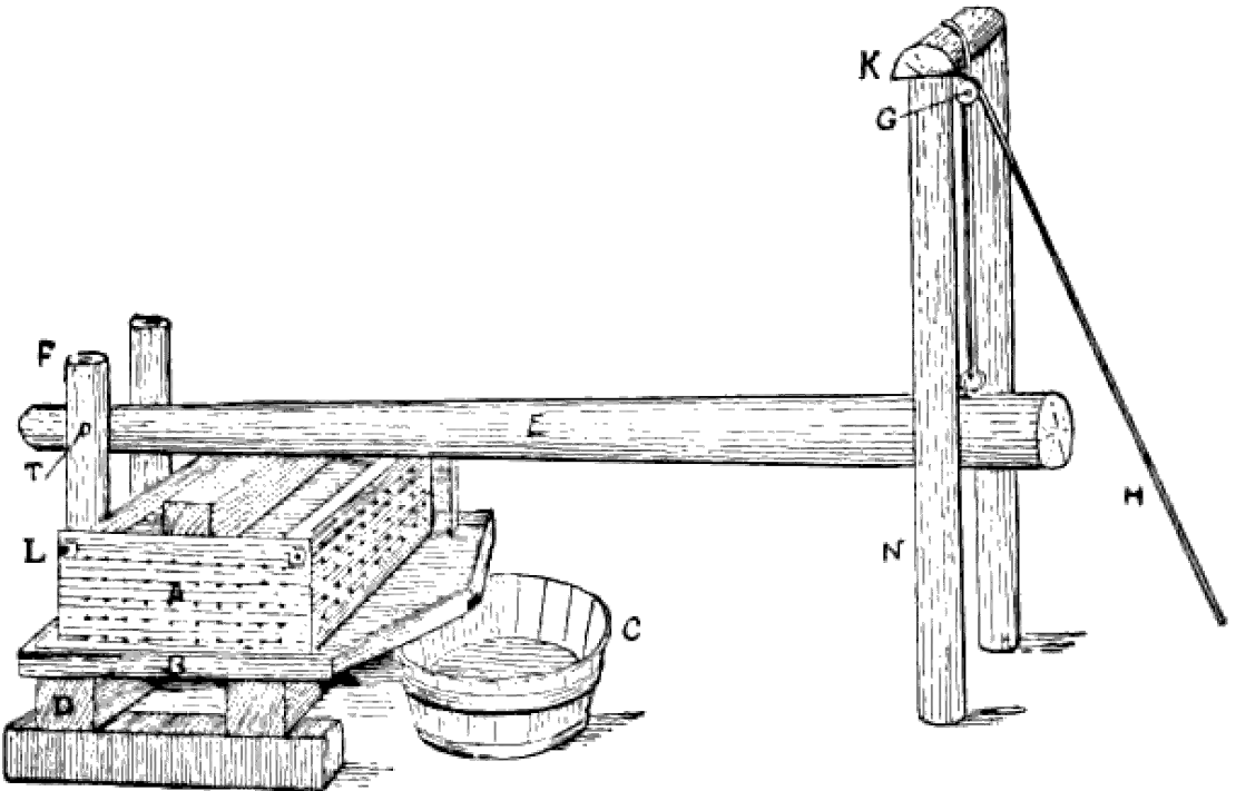
FIG. 69.—Construction of a homemade fruit press.
