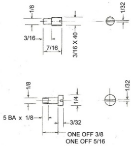
PIVOT SCREWS
