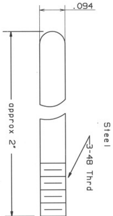
Lifter Rod
