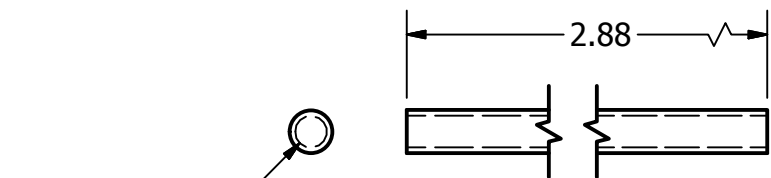
TIE ROD, CYLINDER
