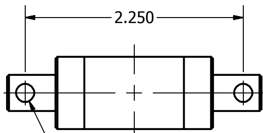
2X Ø.189 THRU S.F. FOR PIN Piston Center
