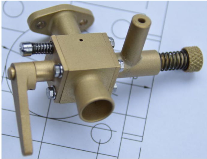
Wyvern carb based on Stride/Rupnow design – light sand blast finish
