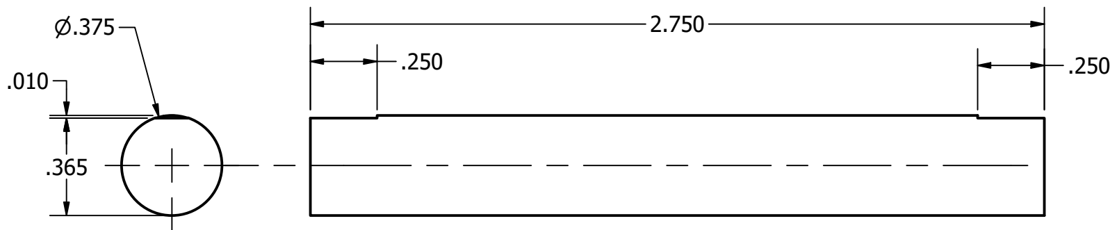
Crankshaft - 02
