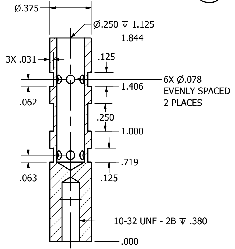
SECTION A-A Valve
