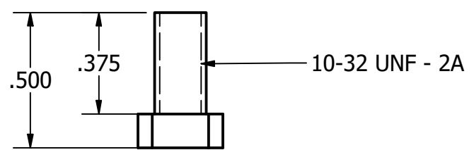
Valve Tappet
