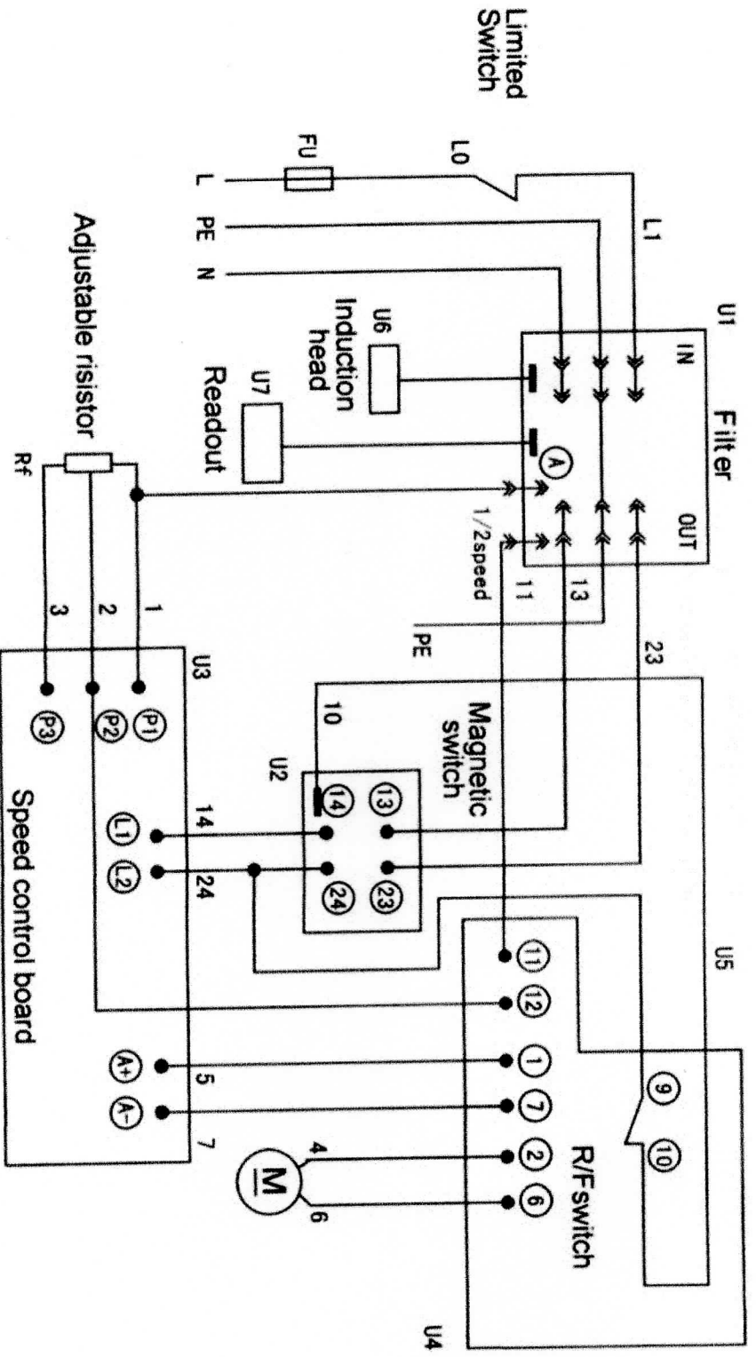
wiring diagram
