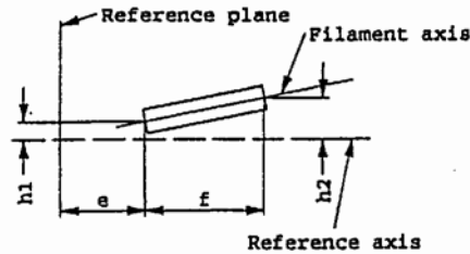
Figure 6 Permissible offset of filament axis (For standard filament lamps only) 2/
