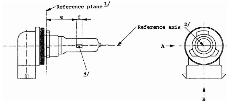
Figure 1- Main drawing
