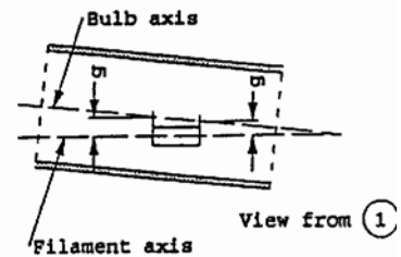
Figure 7 Bulb eccentricity 10/
