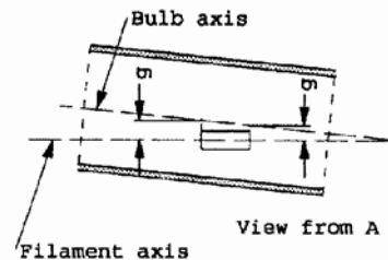
Figure 6- Bulb eccentricity 8/
