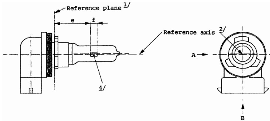
Figure 1- Main drawing
