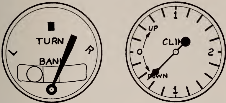
Fig. 15—This Illustration Indicates a Turn, Skidding Out, and Descending.
