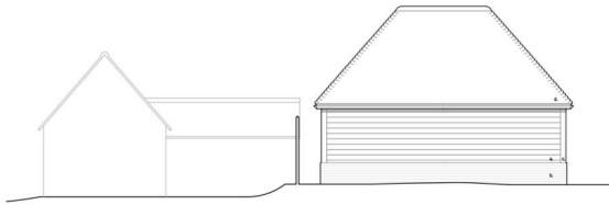
Proposed South East Elevation Scale 1:50
