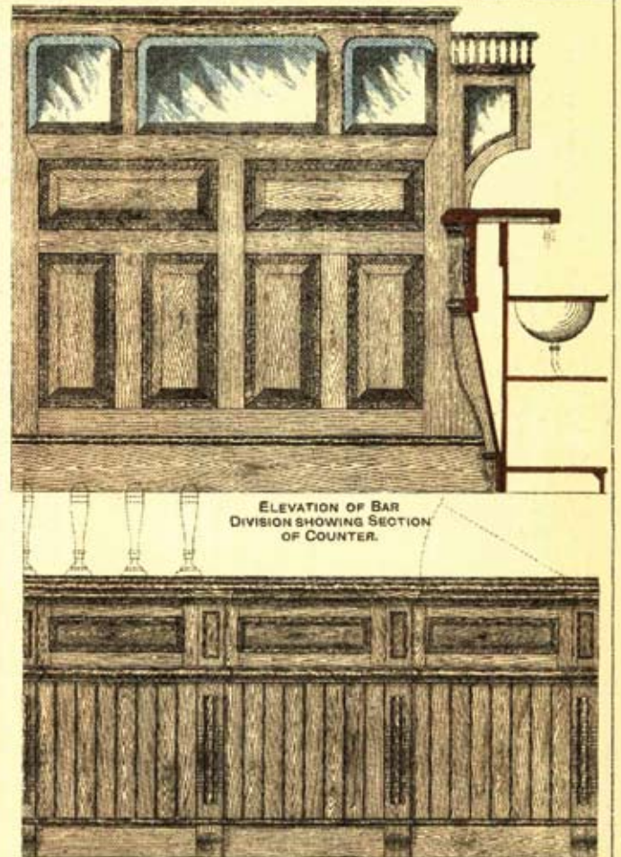
HALF ELEVATION OF BAR COUNTER.
