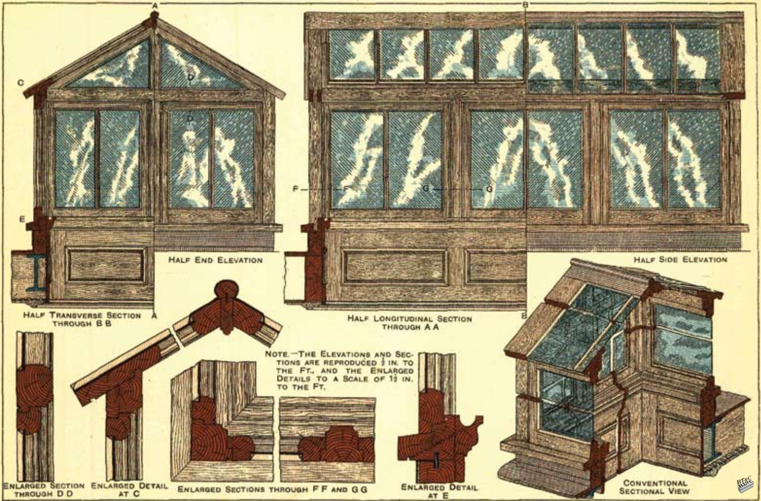
LANTERN LIGHT WITH GABLE ENDS.
