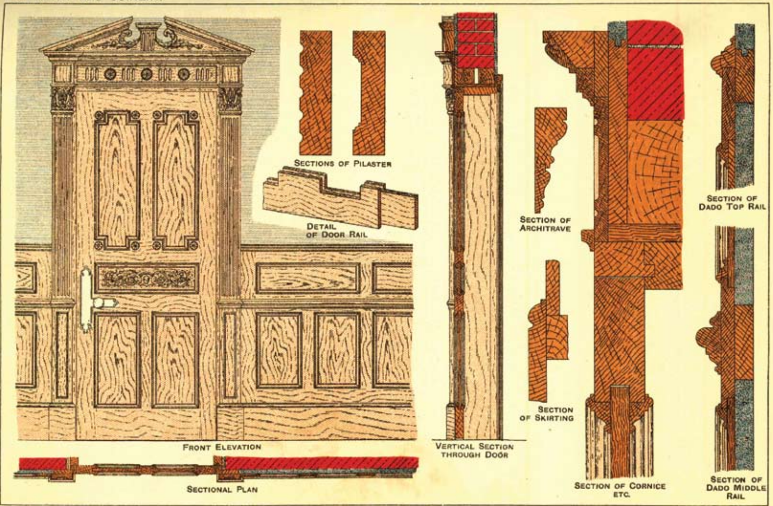
INTERIOR DOORWAY WITH DADO
