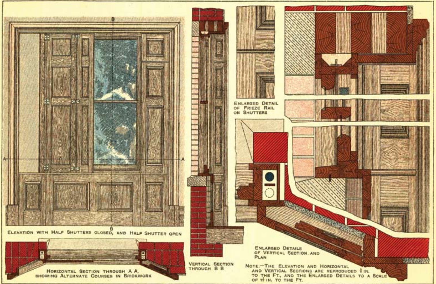
BOXING SHUTTERS TO SASH WINDOW
