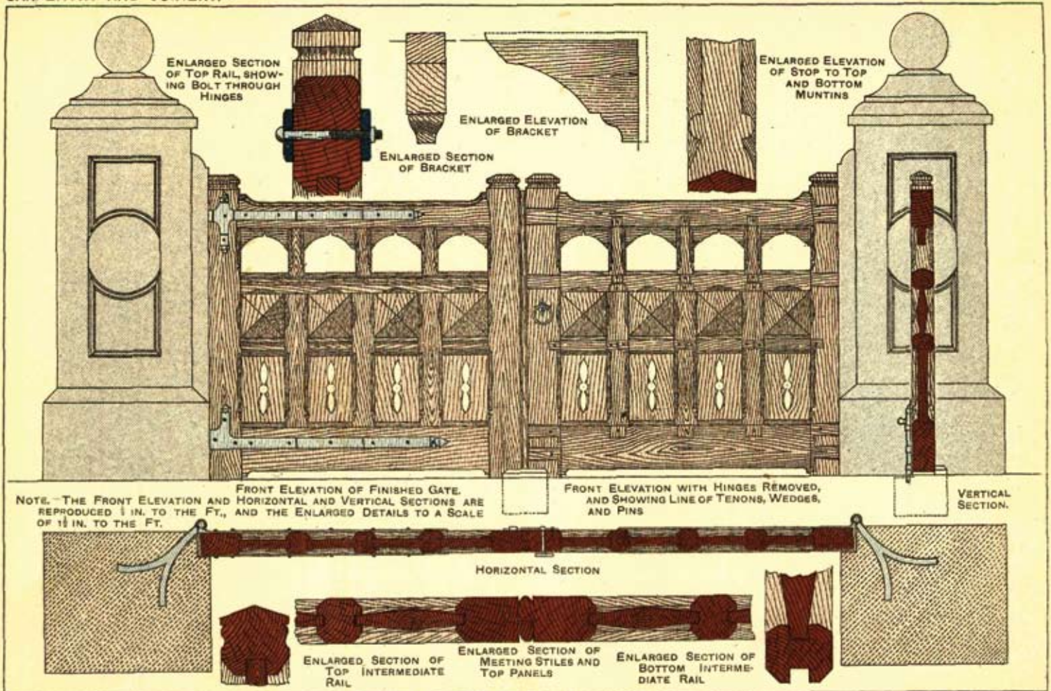
CARRIAGE ENTRANCE GATES.
