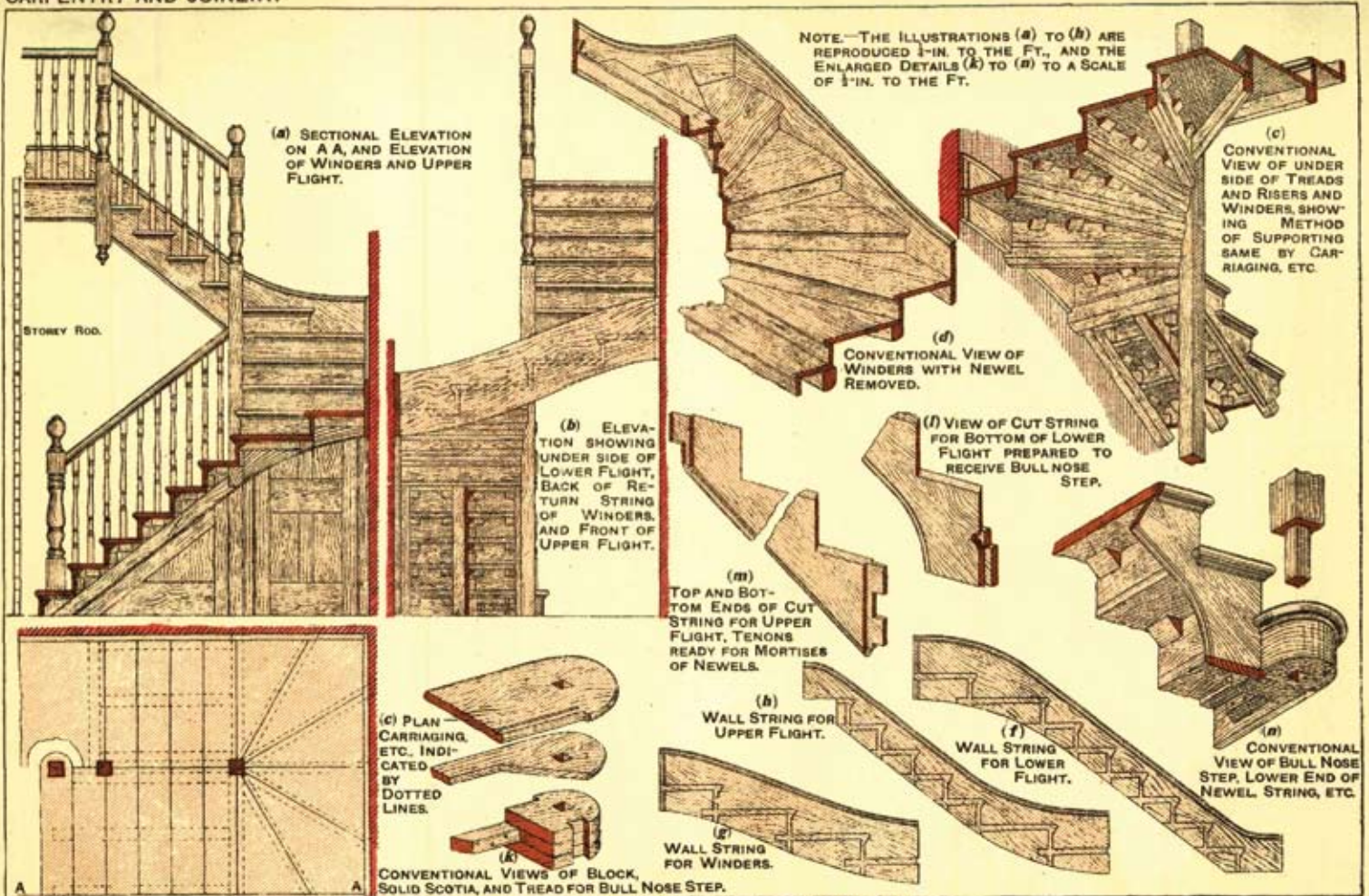
NEWEL STAIRCASE WITH WINDERS IN HALF SPACE.
