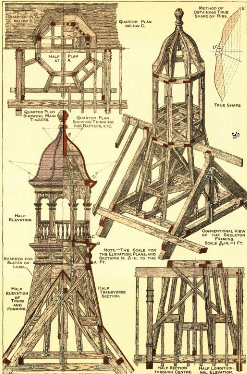
12 CONSTRUCTION OF A BELL OR VENTILATING TURRET FRAMED TO ROOF.
