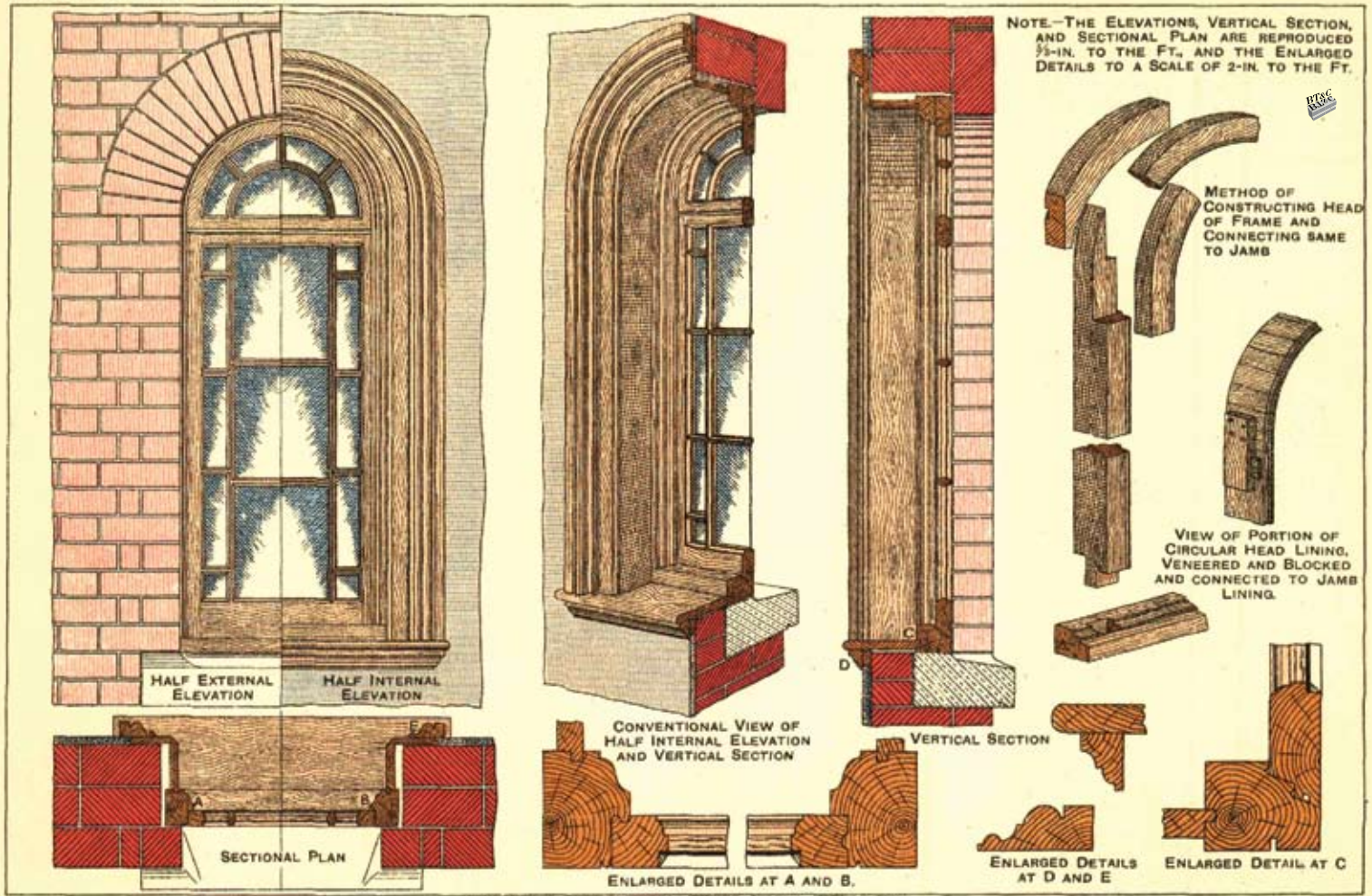
CIRCULAR HEADED CASEMENT WINDOW
